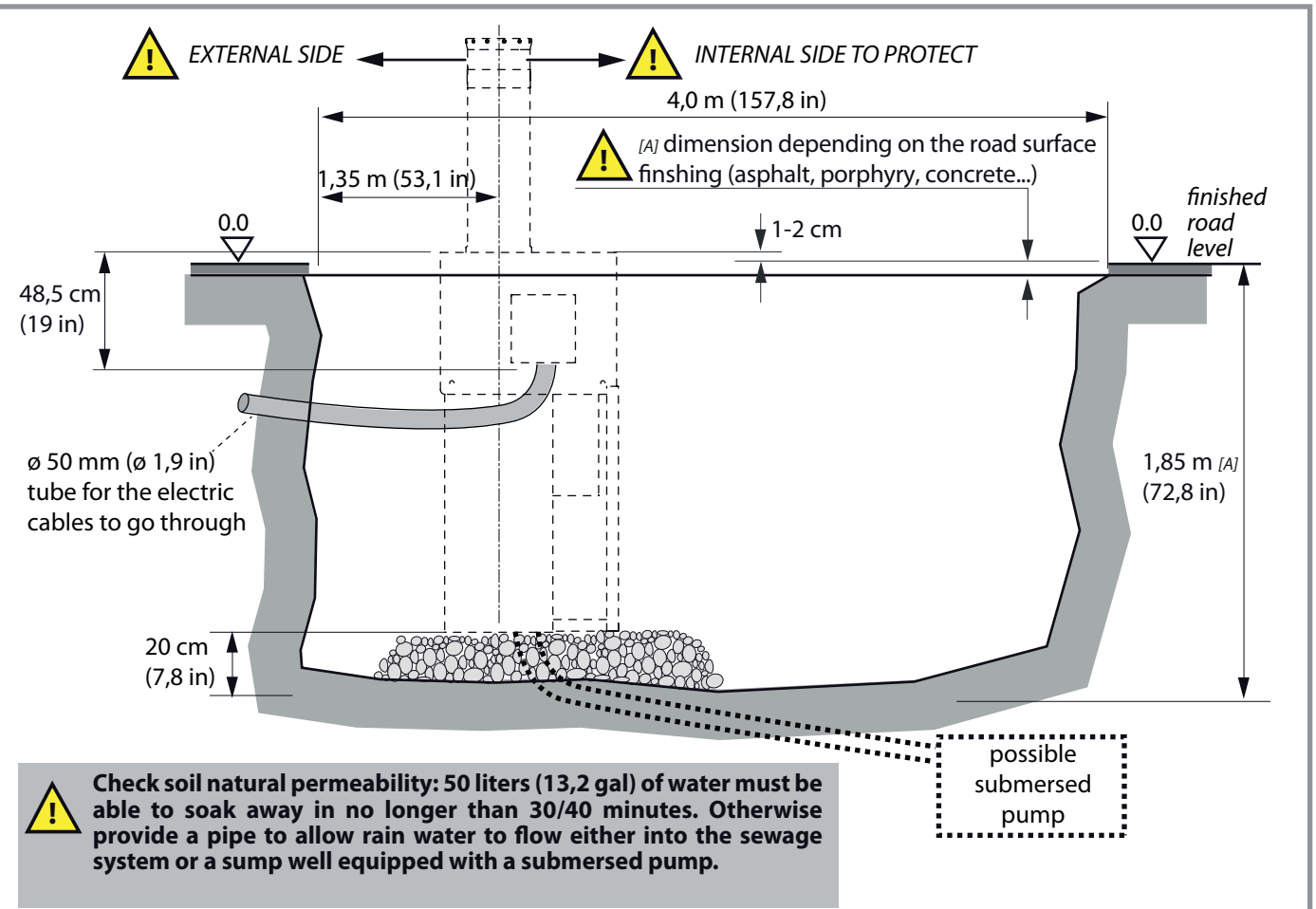
SECTIONAL VIEW
